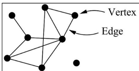
Figure 4. A network with 8 nodes and 10 edges Networks are critical tools used to describe
